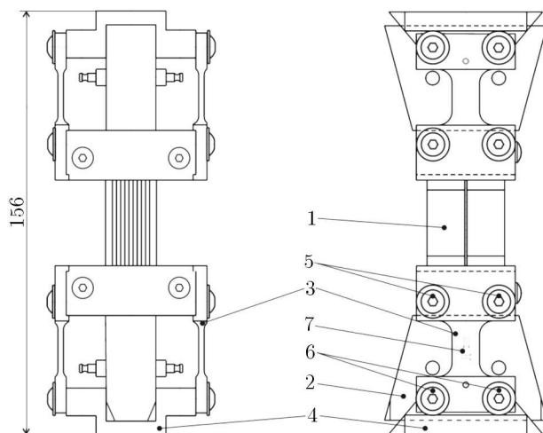
Fig. 2. Technical drawing of the fixture and numbered component parts: front and side view
