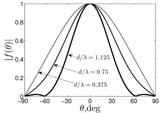
Fig. 5 Directivity function for different values of d/\lambda
