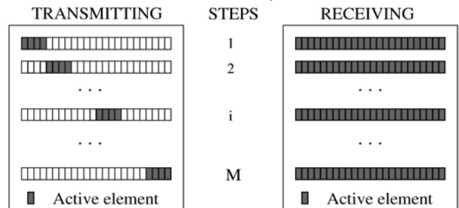
Fig. 3 Transmitting and receiving in the MSTA method
