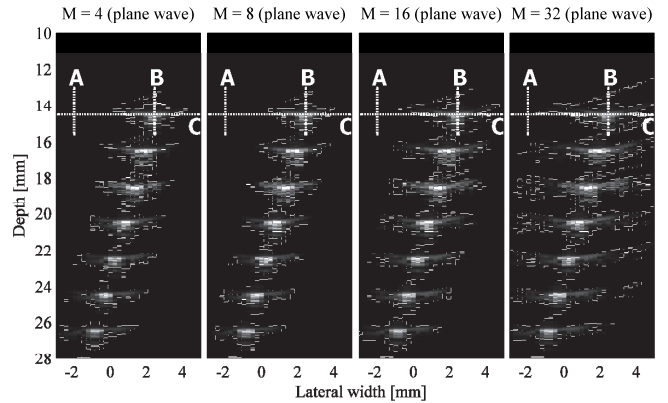
Fig.5. Reconstructed images for plane wave with transmitting aperture in the range from 4 to 32 active elements. Dynamic range is 40 dB for each image
