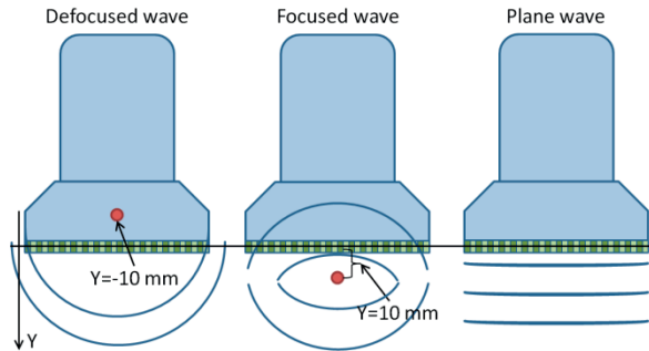
Fig.2. Wave types used in STA testing procedure
