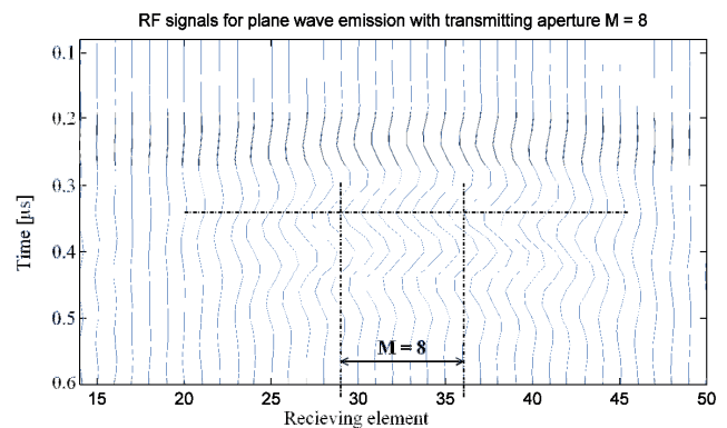
Fig.3. The wave-front shape in plane emission after reflecting from a flat reflector. Size of transmitting aperture is M=8 .
