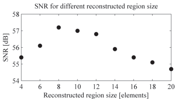
Fig.6. SNR for different reconstruction regions at constant transmitting aperture M = 8 elements
