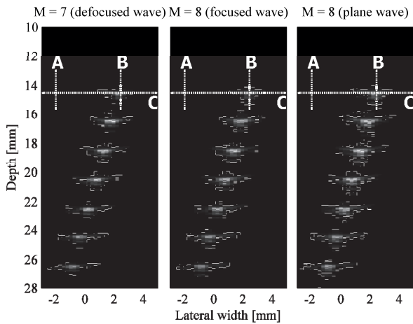
Fig.4. Reconstructed images for a) defocused, b) focused and c) plane waves
