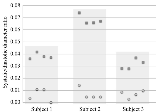
Fig. 5. Comparison of measurements of relative radial artery dilation, SDD = (\text{systolic diameter} - \text{diastolic diameter}) / \text{diastolic diameter} in three volunteers using L40-8 probe (squares symbols) and L14-5 probe (circles symbols) scanning probes, respectively. In all three cases, the calculated average systolic/diastolic dilatation for scanning using L14-5 probe never exceeded 1%, while when using L40-8 scanning probe, the difference between the systole and diastole was clear and averaged 4%, 6.5%, and 3.2%, respectively.
