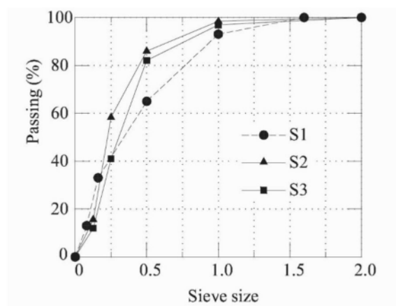
Fig. 1 Sieve curves of the analyzed sands
