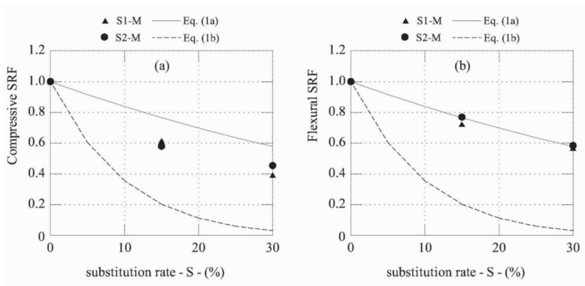
Fig. 11 Comparison between the strength reduction factors (SRF) experimentally measured in M mortars and those obtained by Gregori et al. [32]: (a) compressive strength; (b) flexural strength
