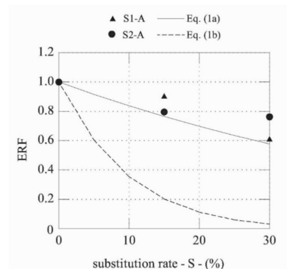
Fig. 12 Expansion reduction factors (ERF) versus Eq. (1a and 1b)
