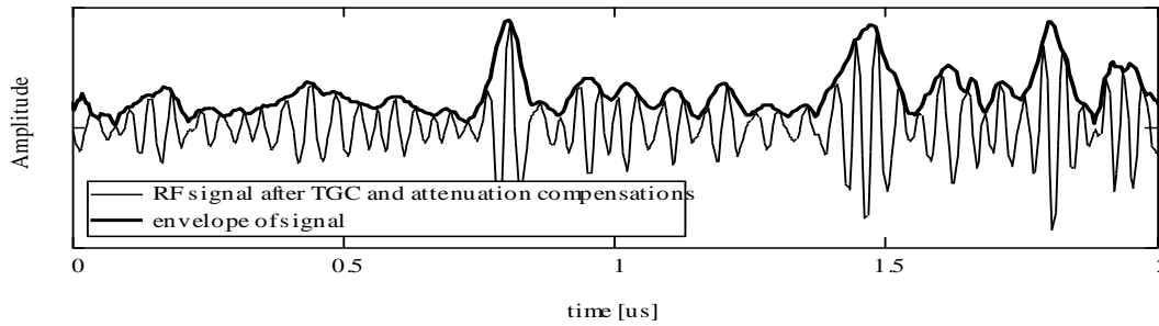
Fig.3. RF signal after the TGC and attenuation compensations and its envelope
