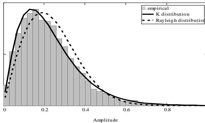
Fig. 4. Theoretical Rayleigh and K distribution and histogram of empirical data obtained at the nape of neck.
