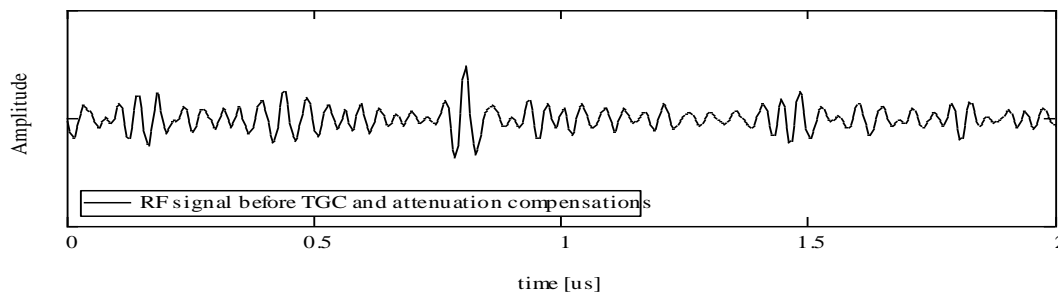
Fig. 2. RF signal before the TGC and attenuation compensations
