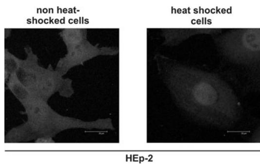
Fig. 2 Subcellular localization of Sgt1 in HEp-2 cells incubated in the presence of leptomycin B. HEp-2 cells were either left untreated or heat shocked. After 24 h cells were stained with anti-Sgt1 antibodies and analyzed by confocal laser microscopy. Bar 20 \mu m
