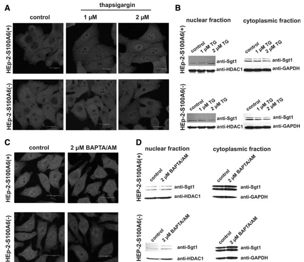
Fig. 4 The changes in subcellular localization of Sgt1 after incubation of HEp-2-S100A6(+) and HEp-2-S100A6(-) cells with 1 and 2 \mu M thapsigargin (TG) (a, b) or 2 \mu M BAPTA/AM (c, d) or 2 \mu M BAPTA/AM (c, d). a, c Immunostaining of cells with anti-Sgt1 antibodies and analysis by use of confocal laser microscopy. Bar 20 \mu m. b, d Western blot analysis showing the level of Sgt1 in the nuclear and cytoplasmic fractions. Staining with anti-HDAC1 and anti-GAPDH antibodies show that each lane contains a similar amount of nuclear or cytoplasmic proteins, respectively
