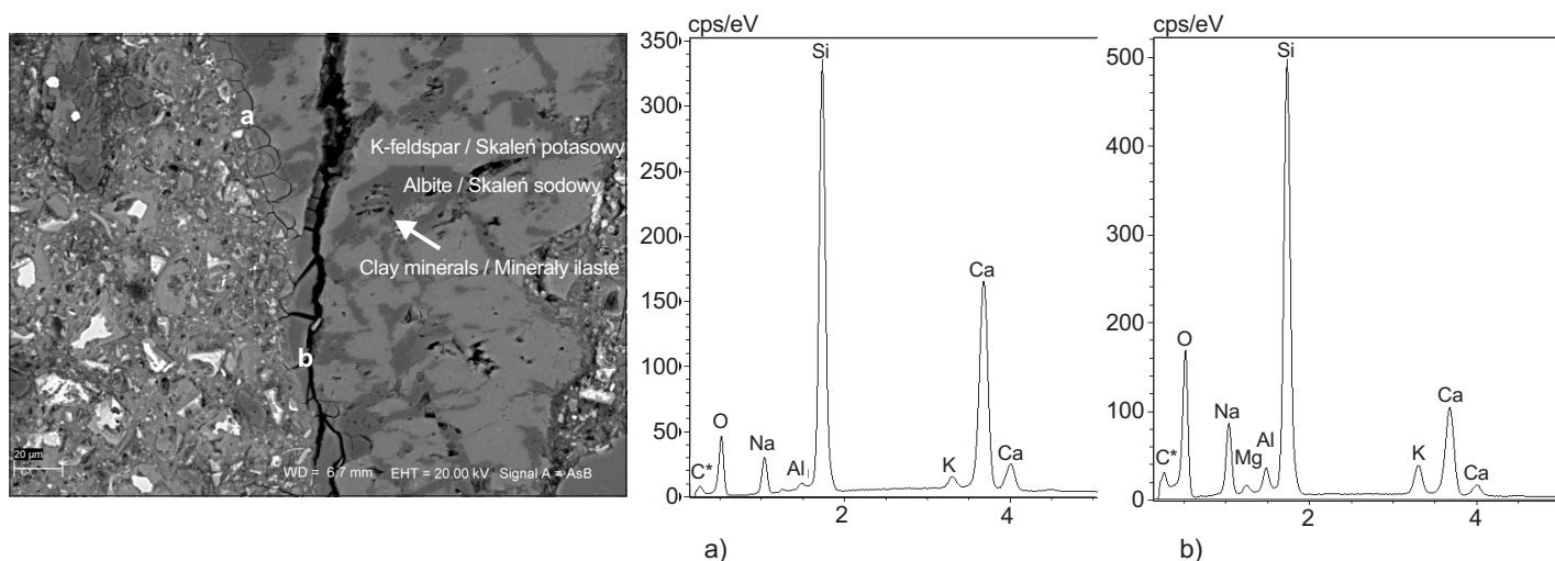
Fig. 12. Microphotograph of a cracked Pr porphyry particle with results of the composition analysis of Si-Ca-Na-K gel in microareas marked (a) and (b)
